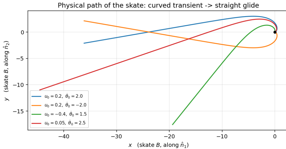
Figure 3: Skate path (x(t), y(t)) for several initial conditions.
