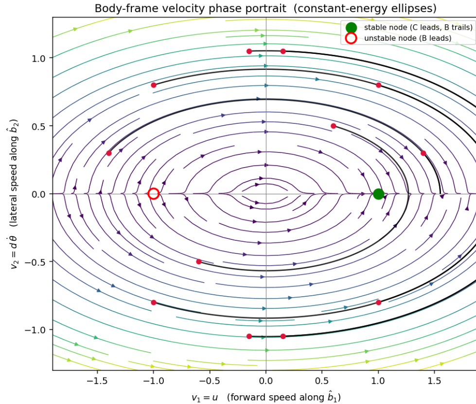
Figure 4: v_2 vs. v_1 for several initial conditions.
